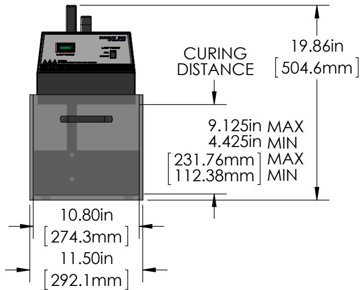
FRONT VIEW WITHOUT REAR SHIELD
