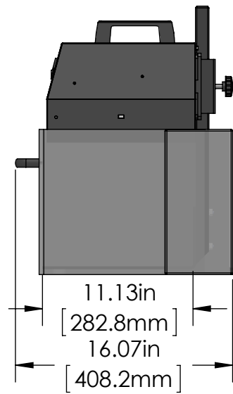
SIDE VIEW WITH REAR SHIELD
