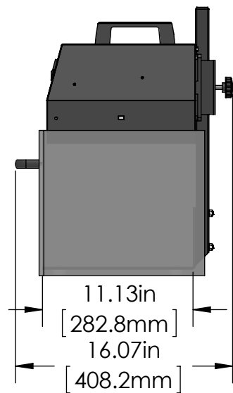
SIDE VIEW WITHOUT REAR SHIELD
