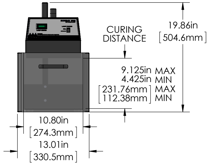
FRONT VIEW WITH REAR SHIELD
